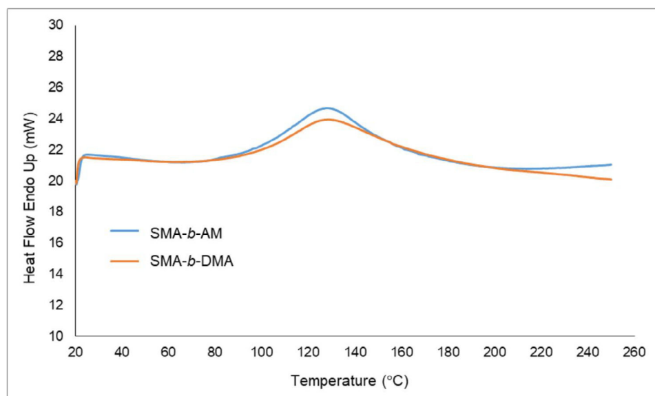
FIGURE 10 DSC thermograms of SMA- b -AM and SMA- b -DMA (heating rate = 10°C/min). AM, acrylamide; DMA, N,N -dimethylacrylamide; SMA, styrene-maleic acid
