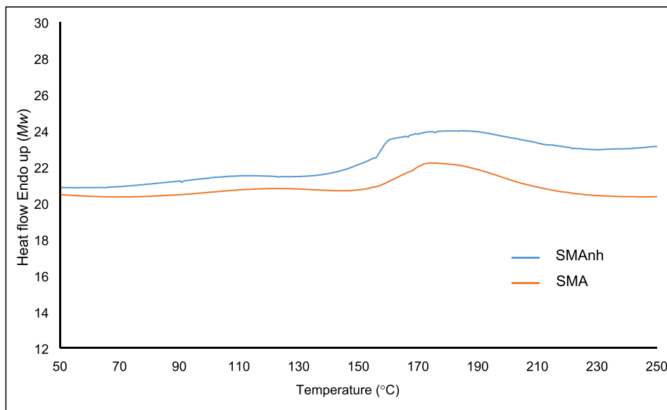
FIGURE 3 DSC thermograms of the SMAnh and SMA copolymers (heating rate = 10°C/min). SMA, styrene-maleic acid; SMAnh, styrene maleic anhydride
