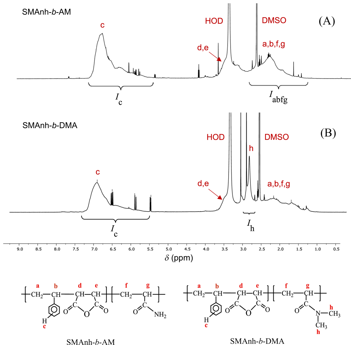
FIGURE 4 ^1\text{H-NMR} spectra of (A) SMAnh- b -AM and (B) SMAnh- b -DMA recorded in d_6 -DMSO as solvent. AM, acrylamide; DMA, N,N -dimethylacrylamide; SMA, styrene-maleic acid; SMAnh, styrene maleic anhydride
