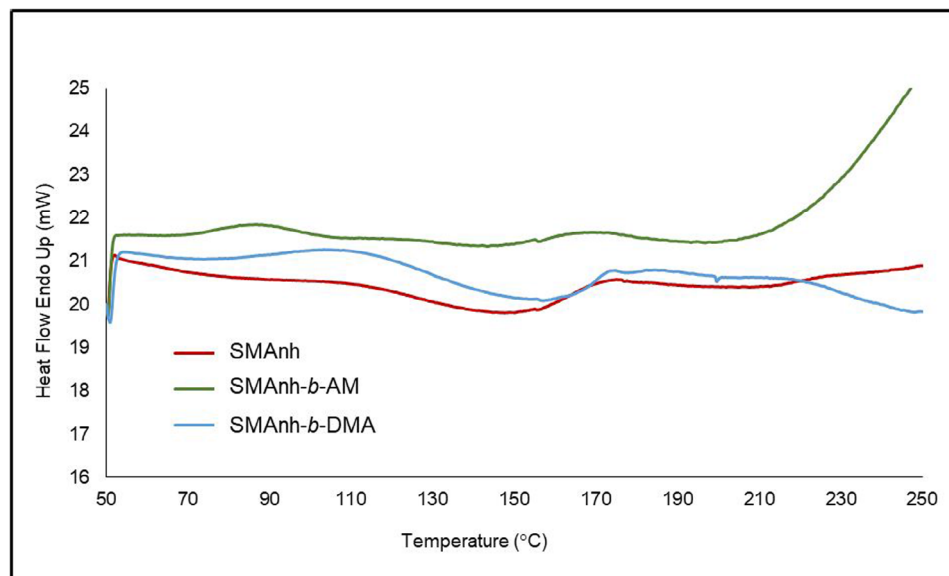
FIGURE 5 DSC thermograms of SMAnh, SMAnh- b -AM and SMAnh- b -DMA (heating rate = 10°C/min). AM, acrylamide; DMA, N,N -dimethylacrylamide; SMA, styrene-maleic acid; SMAnh, styrene maleic anhydride
