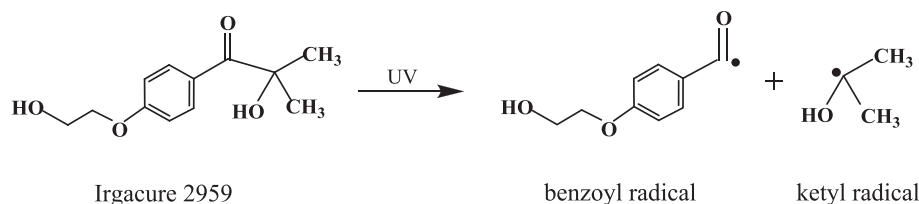
SCHEME 2 Photodissociation of Irgacure 2959
