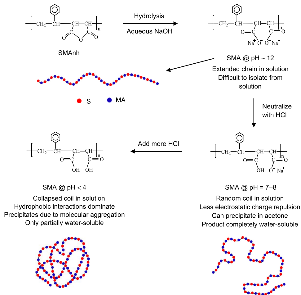
SCHEME 4 pH-dependency of styrene-maleic acid's chain conformation in an aqueous solution
