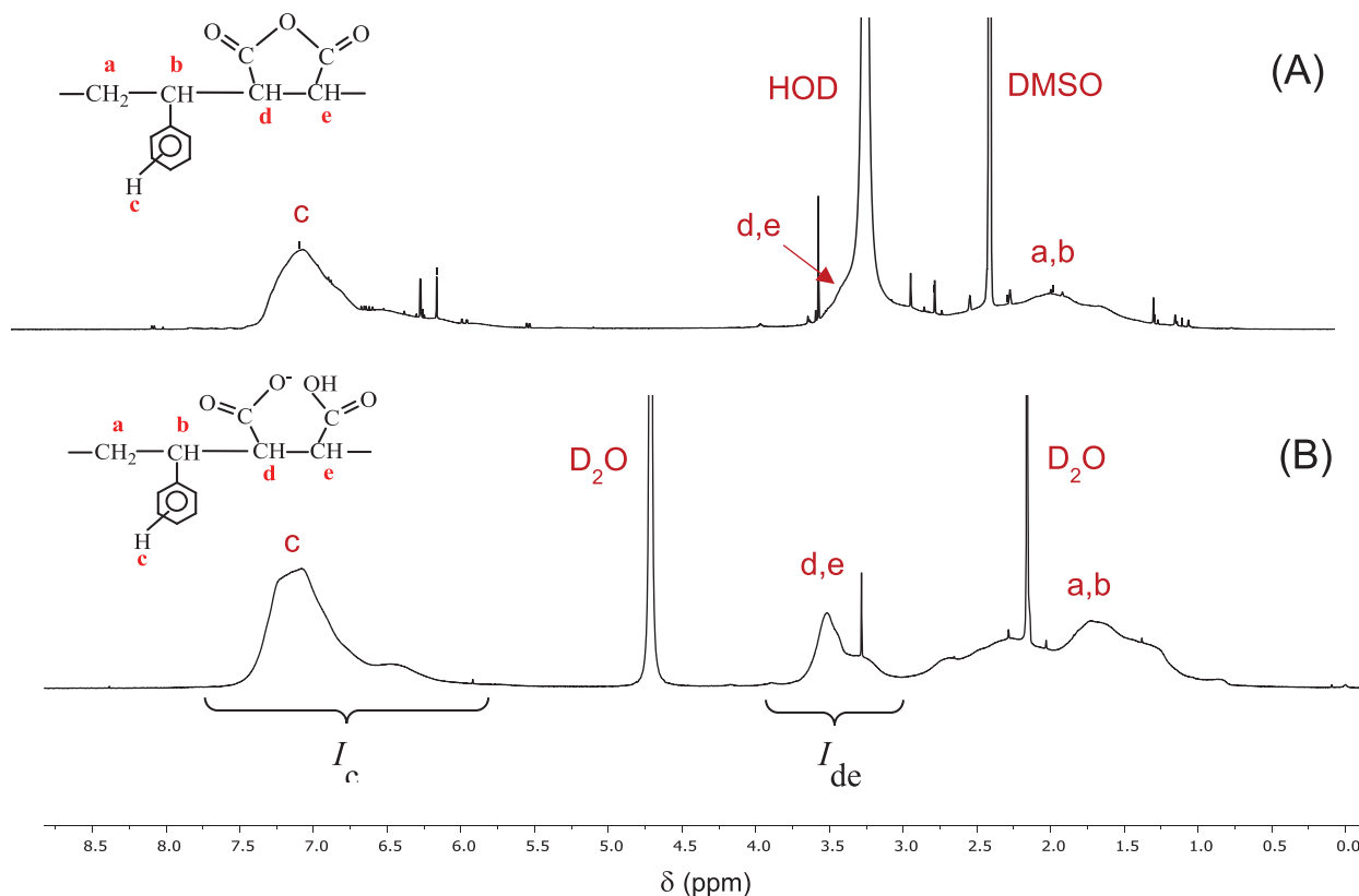
FIGURE 2 ^1\text{H-NMR} spectra of (A) SMAnh recorded in d_6\text{-DMSO} as solvent and (B) SMA recorded in \text{D}_2\text{O} as solvent. SMA, styrene-maleic acid; SMAnh, styrene maleic anhydride
